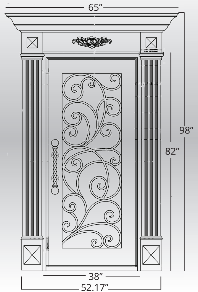
SINGLE DIMENSIONS: 98" H X 65" W
